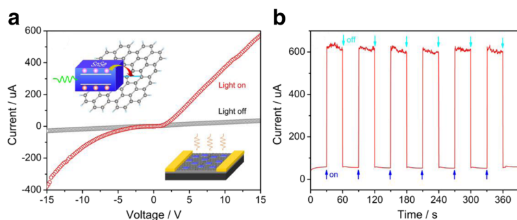
Fig. 6 a The typical I - V characterization of the photodetector device constructed with the SnSe nanoplatform-graphene nanocomposites, the schematic and structural diagram of the photodetector shown in the left upside and right downside inset ; b the photosensitivity of the photodetector device with the voltage of 15 V under the white light or not
