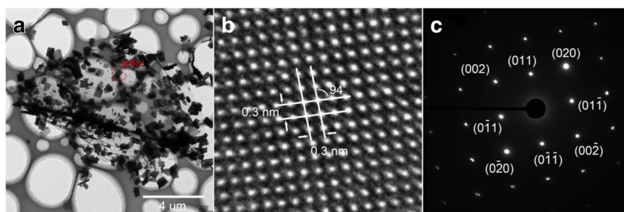
Fig. 3 a The low-magnification TEM image of the representative SnSe nanoplate-graphene nanocomposites; b, c the high-magnification TEM image and SAED pattern of the representative SnSe nanoplate of the rectangular of a , respectively
